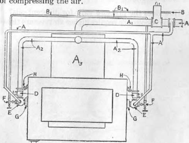
FIG. 2—Typical installation of a multiple spray fuel oil burner in position and piped for using pre-heated air and automatic temperature control. A , uncontrolled cold air from the main air line to the by pass opening on the burner head, the by pass piping around the butterfly air valve on the burner having been disconnected. This by pass air A , is 15 per cent of the total air which passes through the burner, and is sufficient for the low burning position when automatic control is used. This small current of cold air also serves as a blanket protector for the oil tube and spraying parts of the burner from the hot air when a recuperator is used. This protection prevents premature vaporization of the oil at these points, and also the possibility of oil being left in the burner to carbonize and block the channels. A1 , controlled air from the motor operated air and oil valve C ; A3 , recuperator or heat exchanger which heats the air for combustion on its way to the burner, by means of heat from the waste gases from the furnace; A2 , controlled hot air line to the main air opening on the burner; B , oil line from the source of supply to the automatic oil control valve and by pass at C ; B1 , oil supply pipe to the oil control valve F , on the multiple spray burner. All branch lines should be as nearly as possible of equal length; D , butterfly air control valve, built into the burner; E , the burner proper, which sprays the fuel oil and mixes oil and air; G , induced air control. When pre-heated air is used this control is used for lighting only, being closed tightly at all other times. G is machined to fit the body cap of the burner. H , bracket bolted to furnace holds burner in position.
