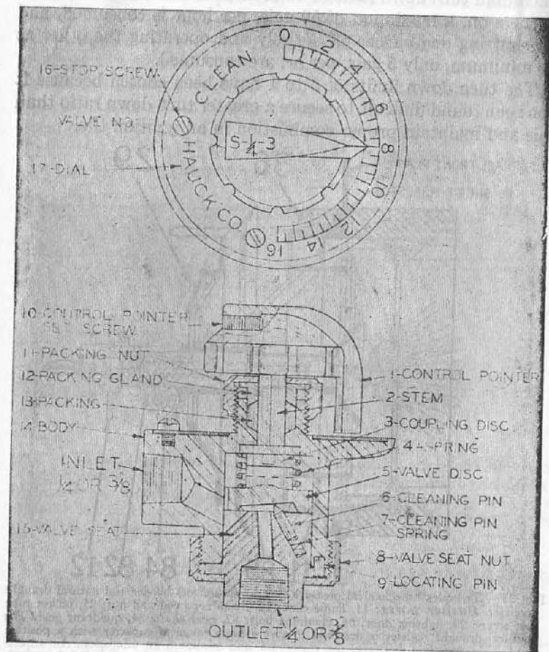
Figs. 39 and 40—Self cleaning valve. In operation , this valve is designed for controlling the flow of oil to burners so that constant accurate combustion conditions can be maintained and easily secured from day to day by setting the valve pointer at the same position. The sludge, dirt and foreign particles that normally build up in the controlling opening of the control valves to reduce the flow are automatically removed in this valve
