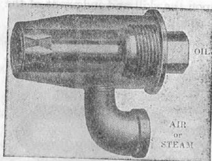
FIG. 24—Venturi high pressure oil burner (phantom view.) Designed for air or steam at 30 lbs. per sq. in. gauge pressure and higher, and for oil from 5° Baume up, the heavier grades require pre-heating.
