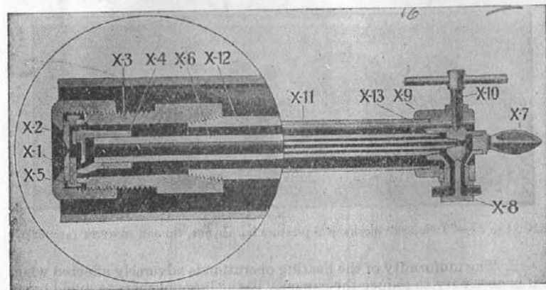
FIG. 33—"Twinplex" mechanical pressure sprayer (atomizing) burner. Wide range type. The parts are: X1, Tip; X2, nut; X3, body; X4, min. atom; X5, max. atom; X6, inner tube; X7, handle; X8, union bushing; X9, housing; X10, housing screw; X11, jacket tube; X12, outer tube; X13, housing body.
